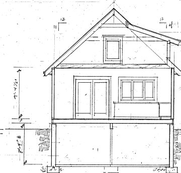
SECTION LOOKING SOUTH
