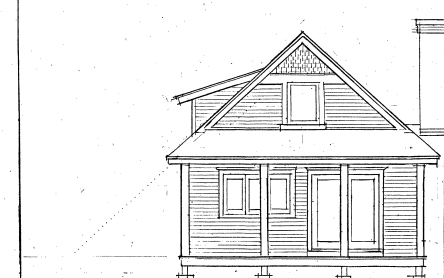
EAST ELEVATION
