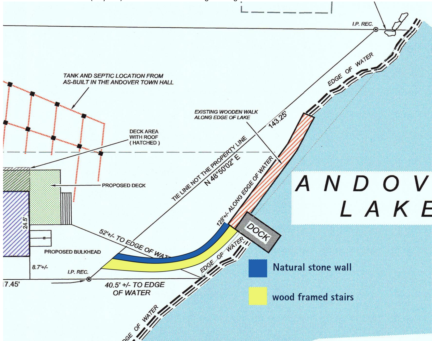
2- Site plan for proposed wall and stairway construction/replacement.
