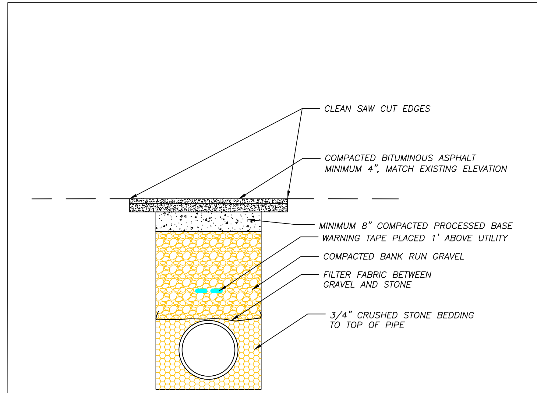
TRENCH DETAIL NOT TO SCALE
